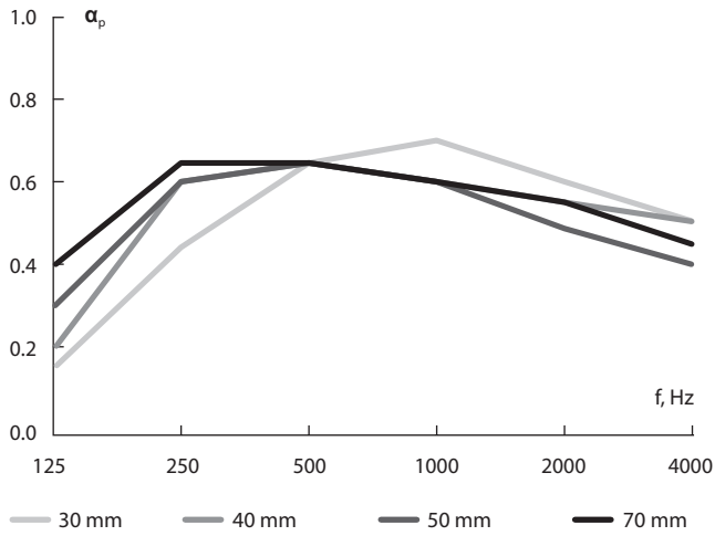
Solid ceilings (on concrete)
