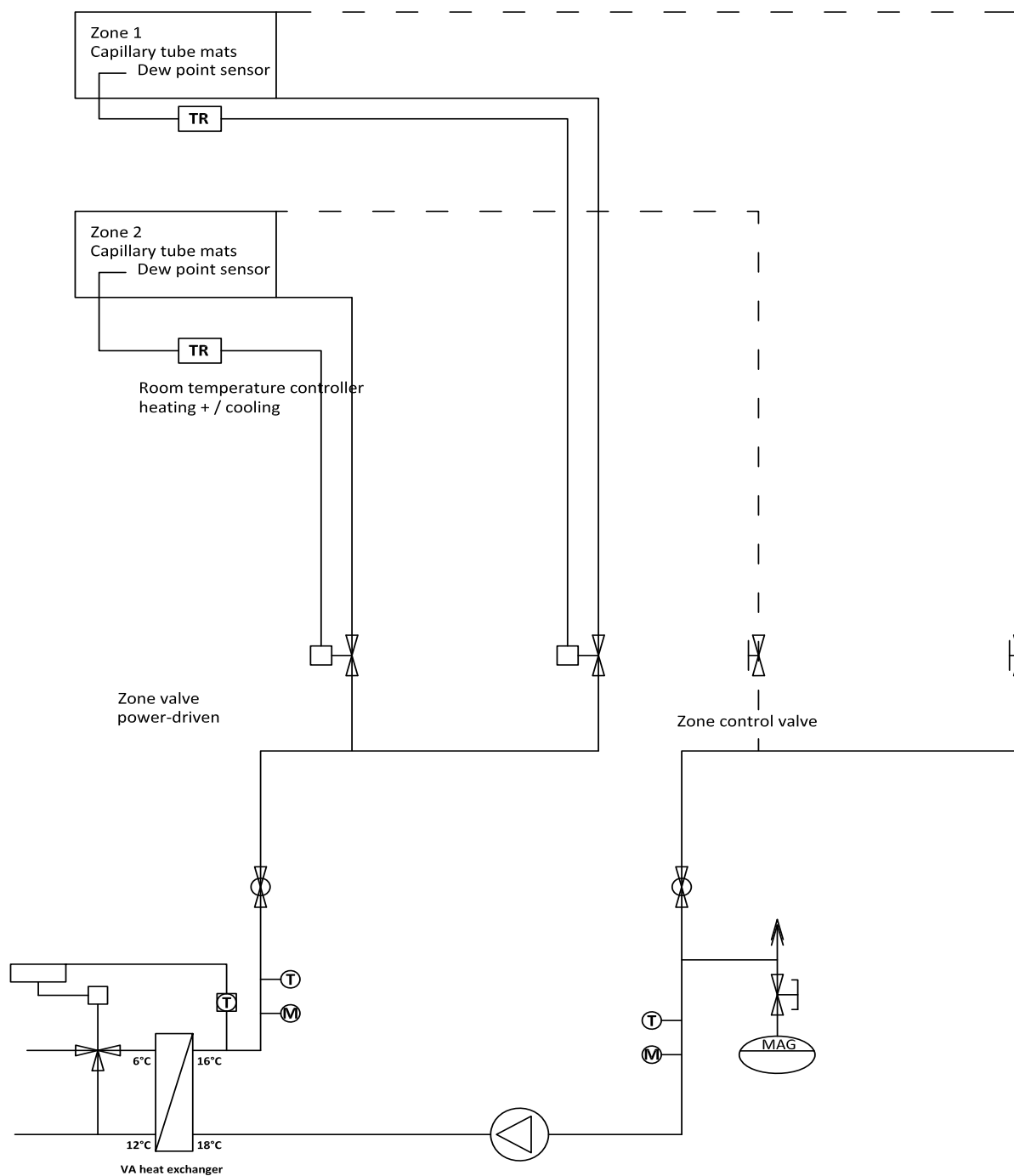
Schematic diagram: Capillary tube system cooling (temperature example)
